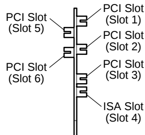
Riser Board Slot Configuration (End View)
